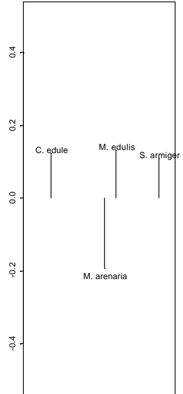
factor loadings trend 3
