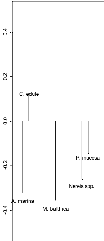
factor loadings trend 1
