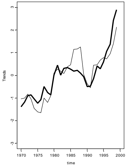
DFA1 and PPCA1
