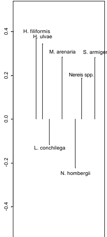
factor loadings trend 2
